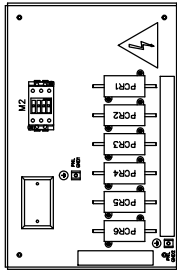
PRECHARGE PANEL DETAIL SCALE 3 : 1
