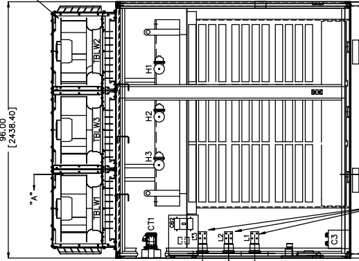
FRONT VIEW W/DOORS REMOVED
